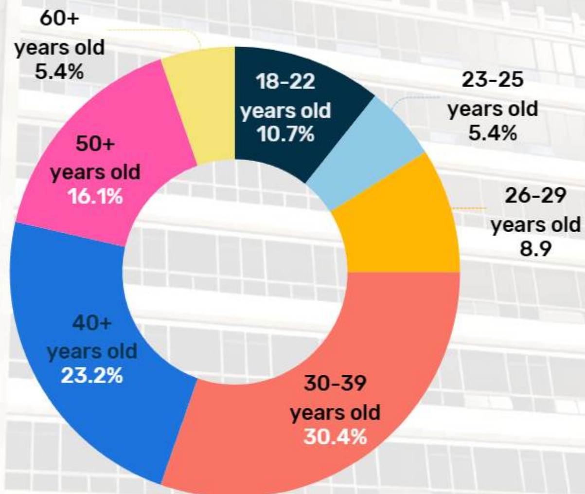
AGE RATIO
