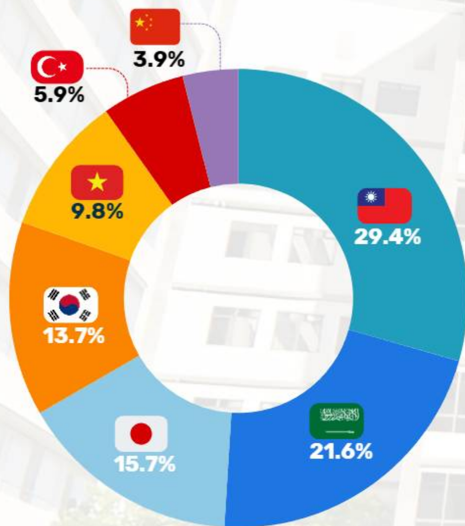
NATIONALITY RATIO
